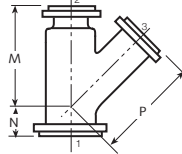
45° Lateral Reducing on Run and Branch
