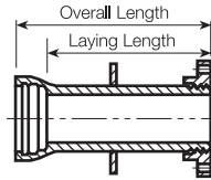
Fastite-Thrust Collar-Flange
