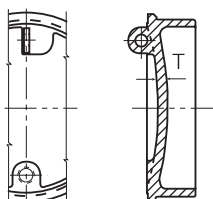
54"-64" Lok-Ring Plugs
