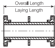
Flange-Thrust Collar-Flange
