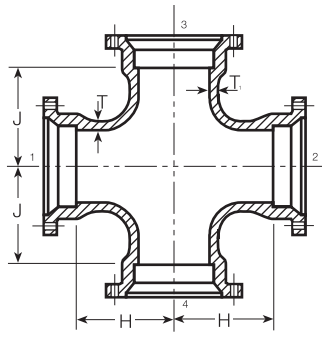
All MJ Cross
