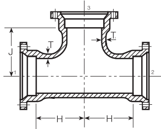
All MJ Tee
