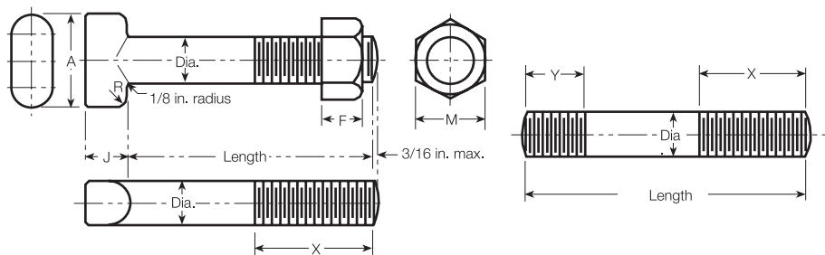
Tee Head Bolt
