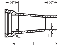
A-225 Large End Bell Reducer
