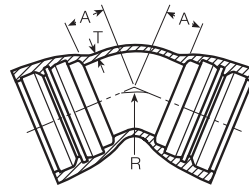
Lok-Ring Bell-Bell**
