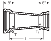
A-224 Bell & Bell Reducer
