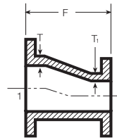
Eccentric Reducer
