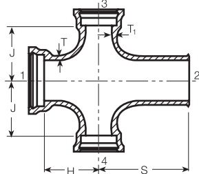
A-21 Bell - Spigot - Bell & Bell
