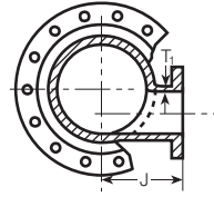
A-30127 MJ, MJ and Flg Blow-Off Branch
