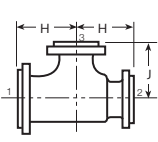
Tee Reducing on One Run and Branch
