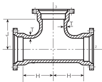
All MJ Tee
