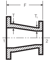
Concentric Reducer
