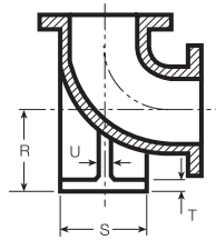
Short Radius AWWA C110
