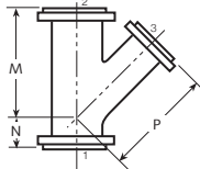
45° Lateral Reducing on Branch
