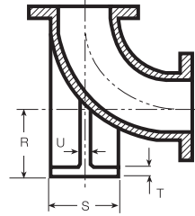
Long Radius AMERICAN Standard
