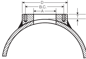
A-96946 Welded-On Boss Faced and Tapped for AWWA C110 or C115 Flange Connection
