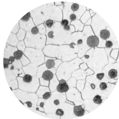
Photomicrograph showing graphite form in ductile iron.
