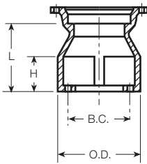
A-10752 MJ Sludge Shoe
