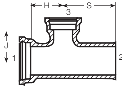
A-115 Bell - Spigot & Bell Tee
