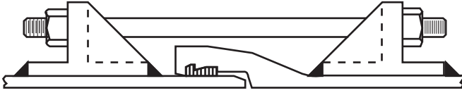
Lugged Fastite Joint
