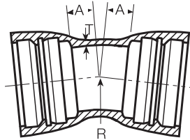
Lok-Ring Bell-Bell**
