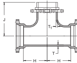
MJ and Swivel Tees
