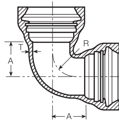
Flex-Ring Bell-Bell**
