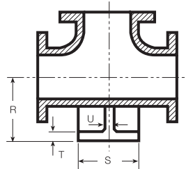
Base Tee
