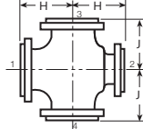
Cross Reducing on Run
