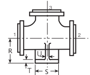
Base Tee
