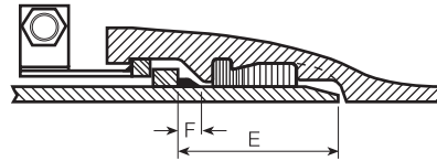
Lok-Ring® Joint
