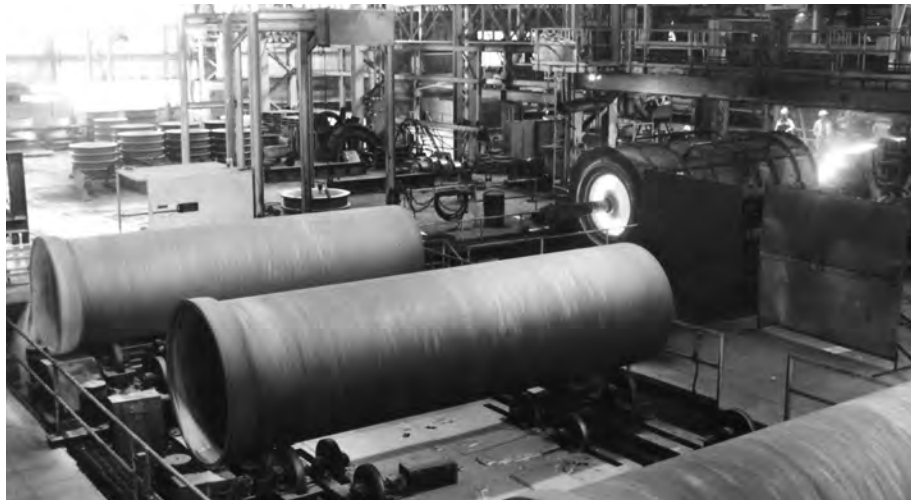
View of modern plant where the large-diameter sizes of pipe are centrifugally cast in nominal 20-foot lengths by the deLavaud process.
