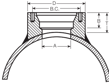
A-96945 Welded-On Boss Drilled and Tapped for AWWA C111 Mechanical Joint Connection
