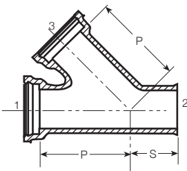
A-123 Bell, Spigot & Bell Wye
