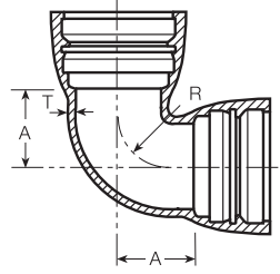
Lok-Ring Bell-Bell**
