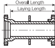
MJ-Thrust Collar-Flange
