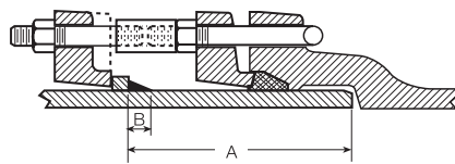
MJ Coupled Joint
