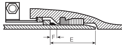
Lok-Ring® Joint
